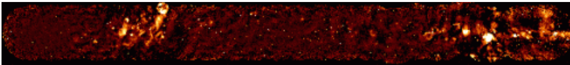
Figure 6-4: The galactic Plane imaged at 327 MHz. for Deuterium by the WRST galactic plane survey. See: www.ucalgary.ca/ras/WRSTsurvey .
