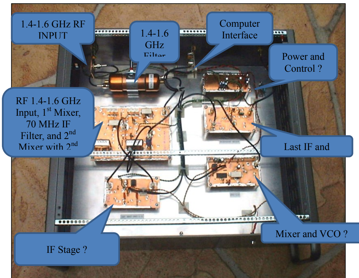
Figure 4-7: Internal view of the SpectraCyber Receiver for H I (1.4 GHz) and OH MASER (1.66 GHz) reception, being of an internal modular construction of the 3rd-order superheterodyne receiver. Photo, courtesy Jeff Lightmann & Carl Lyster, Radio Astronomy Supplies
