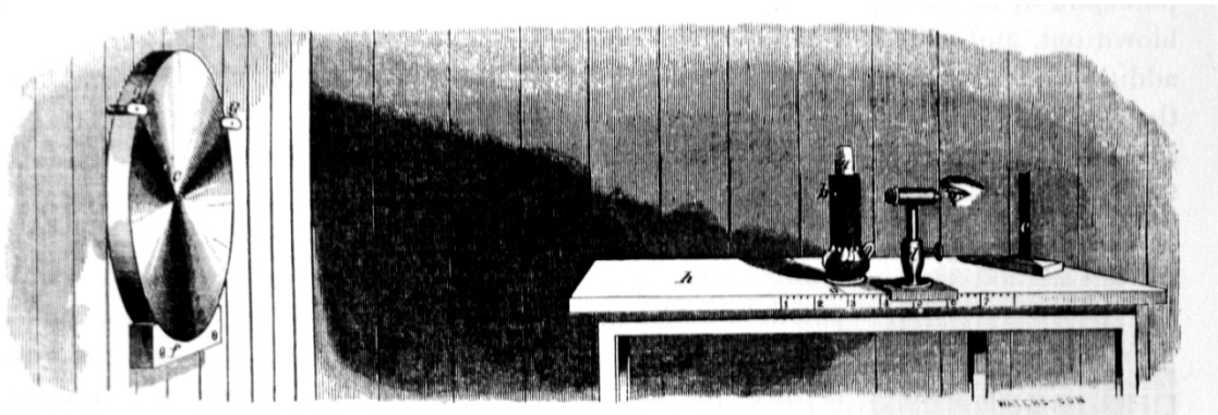
Fig. 23 – Draper's depiction of his modified Foucault test (from, "On the Construction of a Silvered Glass Telescope" - 1865). Note the ruled scale on the table-edge near the observing position; this allowed for accurately measuring the distances to the various zones on the mirror.
